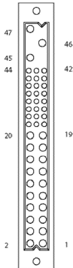
Figure 4. Mating connector
